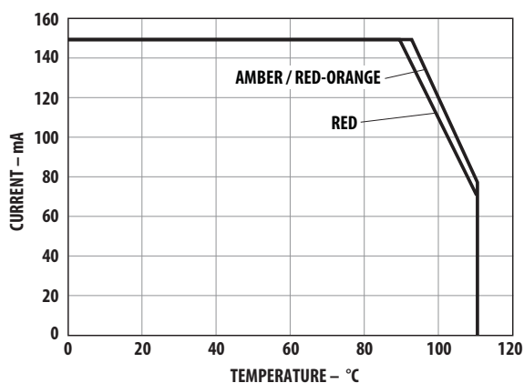
Figure 6b. Maximum forward current vs. solder point temperature. Derated based on T_{JMAX} = 125^{\circ}\text{C} , R_{JP} = 60^{\circ}\text{C/W} .
